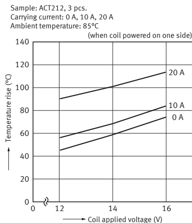
1-2. Coil temperature rise ( at 85 °C )
