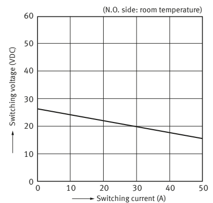
2. Max. switching capability ( Resistive load, initial )
