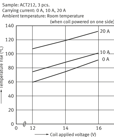
1-1. Coil temperature rise ( at room temperature )
