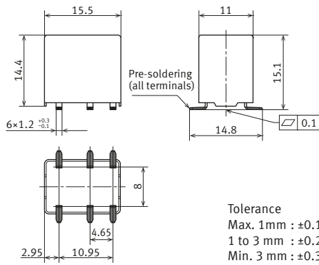
External dimensions
