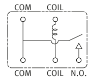
Schematic ( BOTTOM VIEW ) 1 Form A
