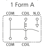
Schematic ( TOP VIEW )
