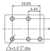
PC board pattern ( BOTTOM VIEW ) 1 Form A
